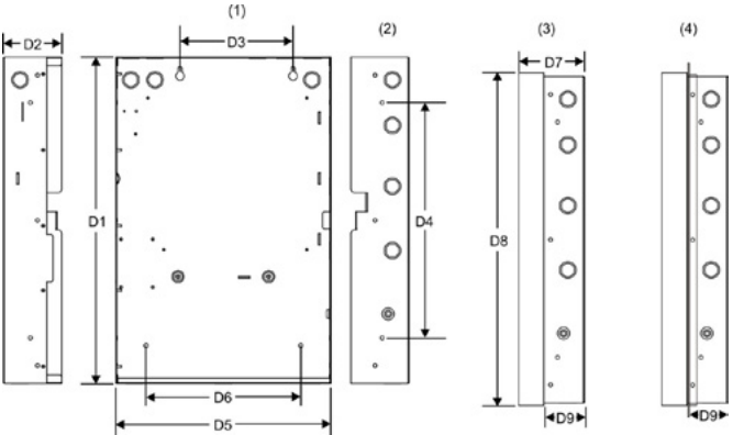
(1) Surface Mounting Holes (3) Backbox with Door Attached (2) Semi-flush mounting Holes (4) Backbox with door and trim kit attached.
